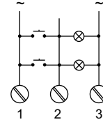
3 wires connection
