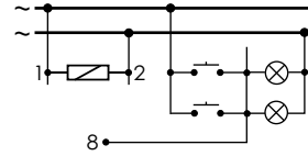
3 wires connection
