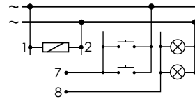
4 wires connection
