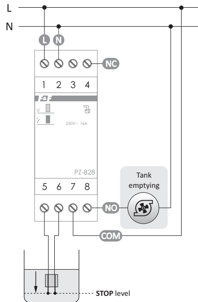
Tank emptying
