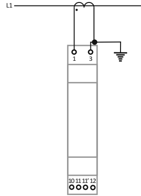
Indirect measurement of current using the current transformers.
