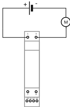
Direct measurement of current DC circuits
