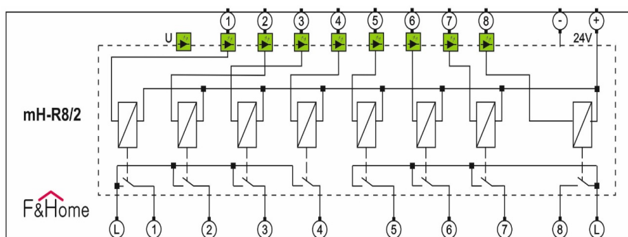
Connection diagram
