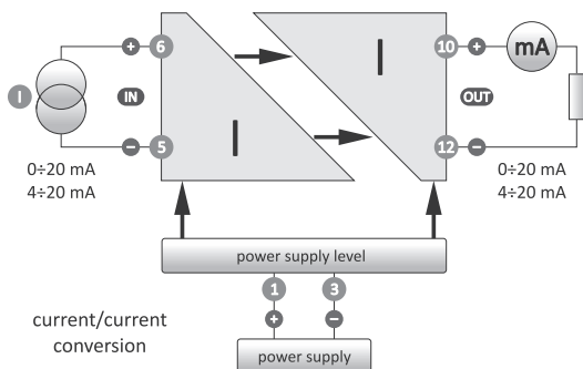
Current/current
