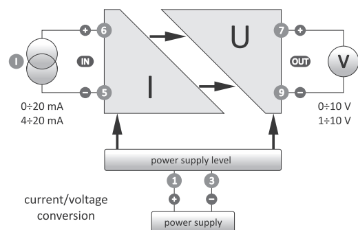
Current/voltage
