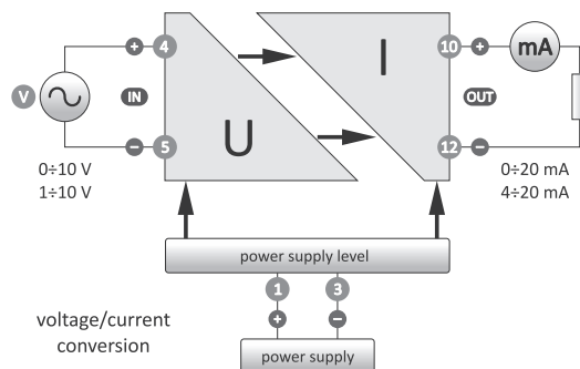
Voltage/current
