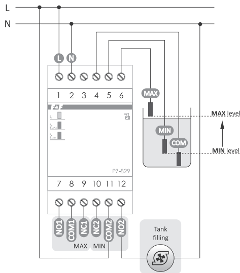
Tank filling
