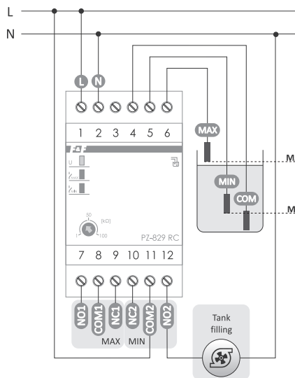
Tank filling
