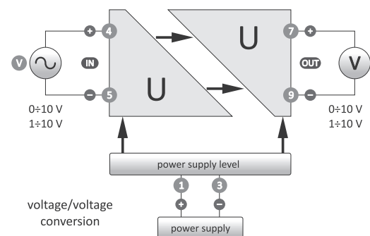
Voltage/voltage
