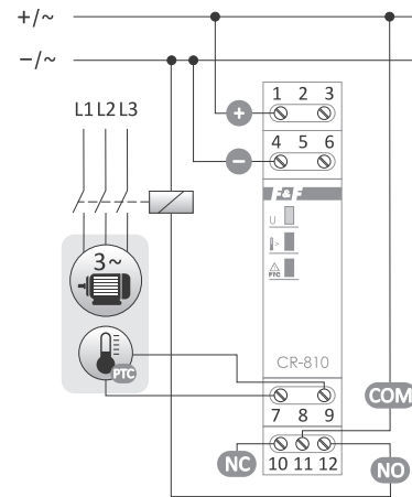
24 V version
