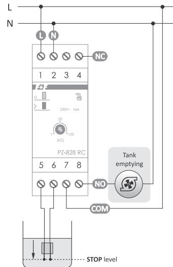
Tank emptying
